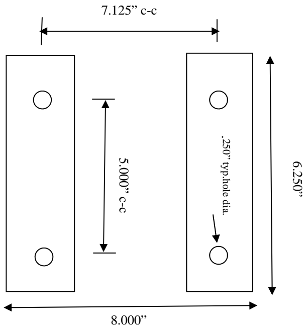
Foot print of bracket when assembled on poly board
